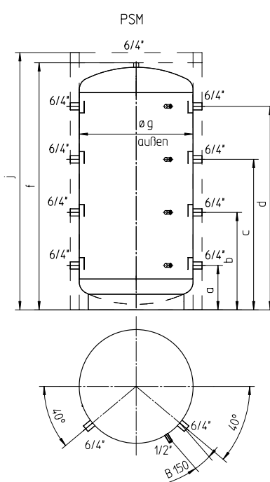
PSM - Bufferreservoir
