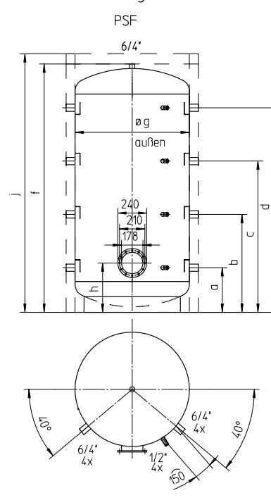
PSF buffer tank Flange D 240
