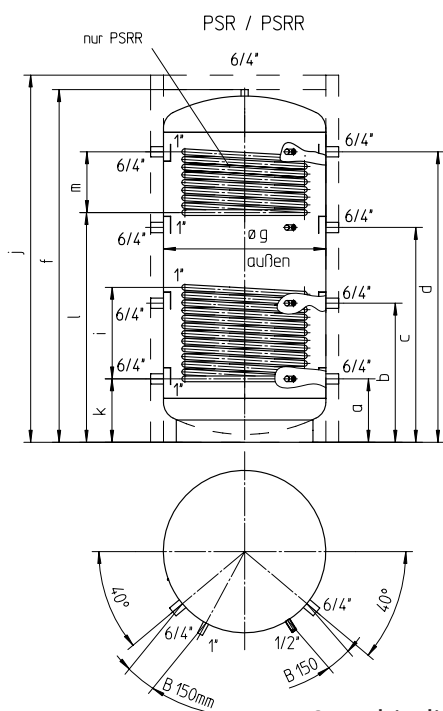
PSR/PSRR - Bufferreservoir buizenraster
